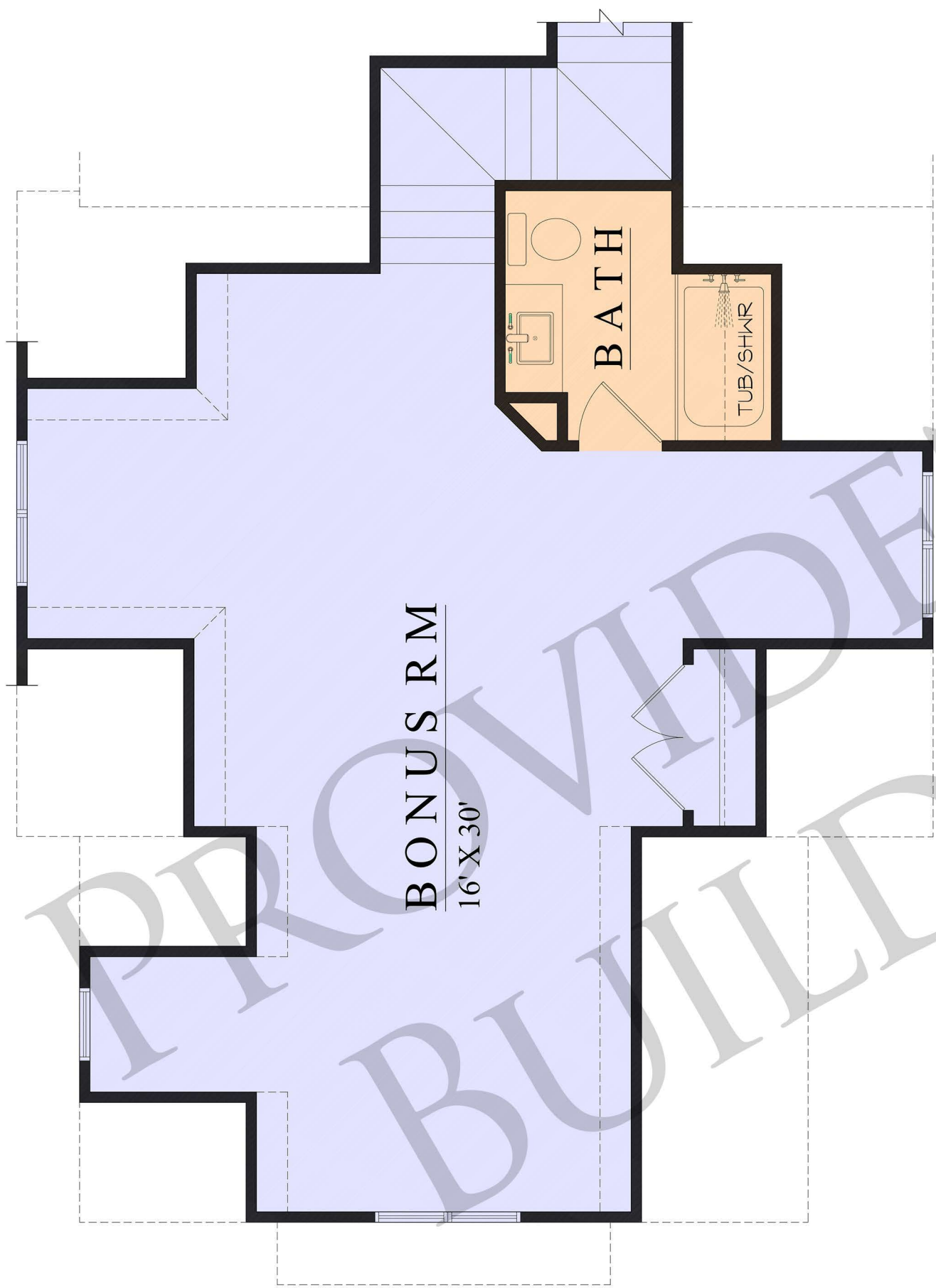
UPPER FLOOR PLAN 624 SQ. FT.
