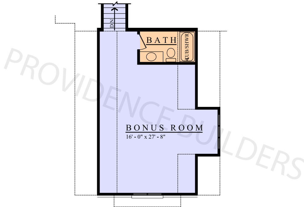
UPPER FLOOR PLAN 480 SQ. FT.
