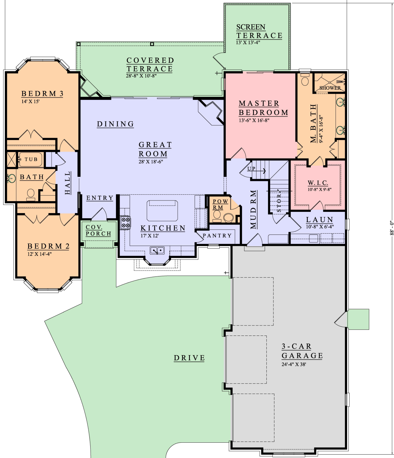
MAIN FLOOR PLAN 2224 SQ. FT.
