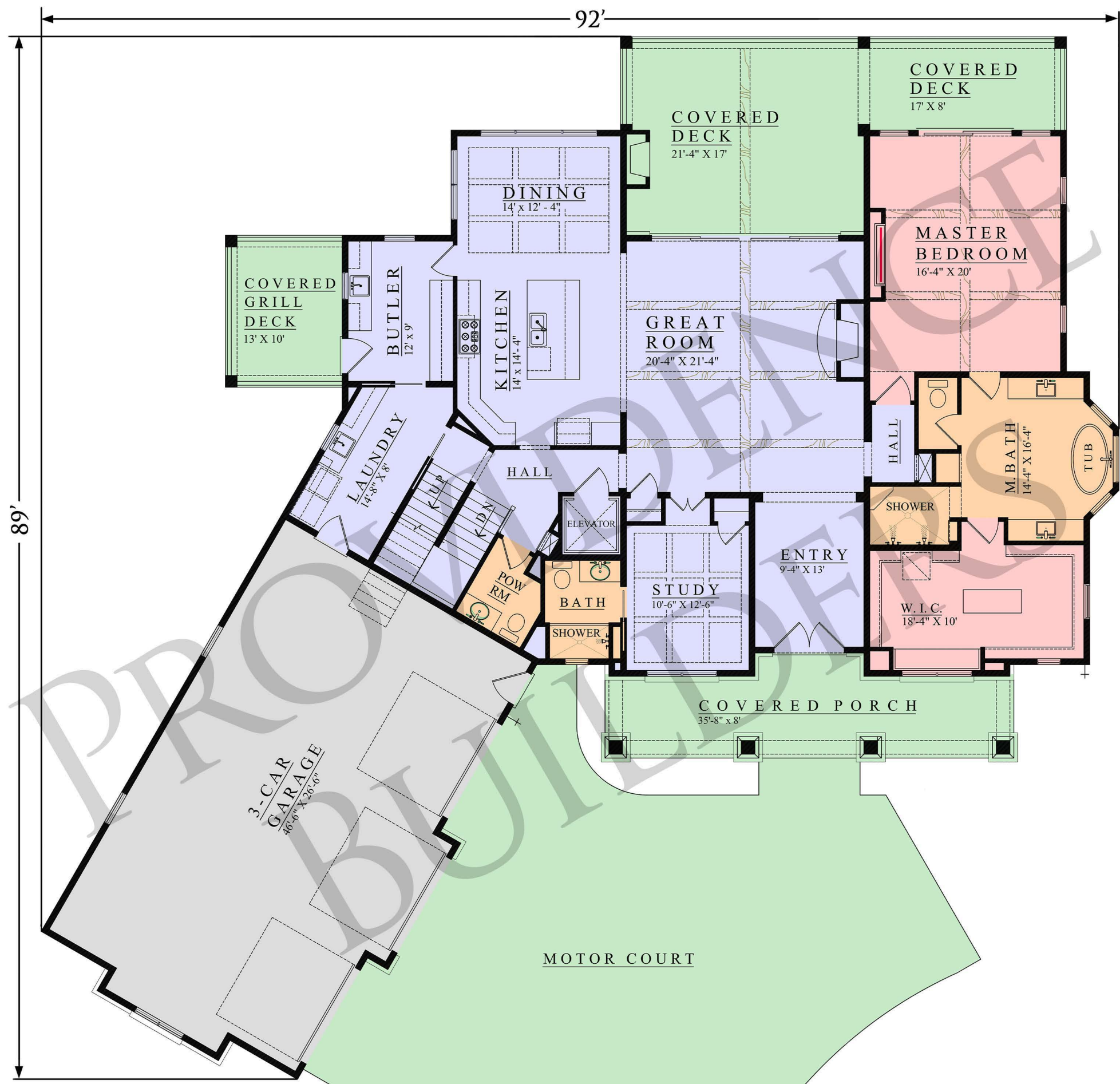
MAIN FLOOR PLAN 2592 SQ. FT.
