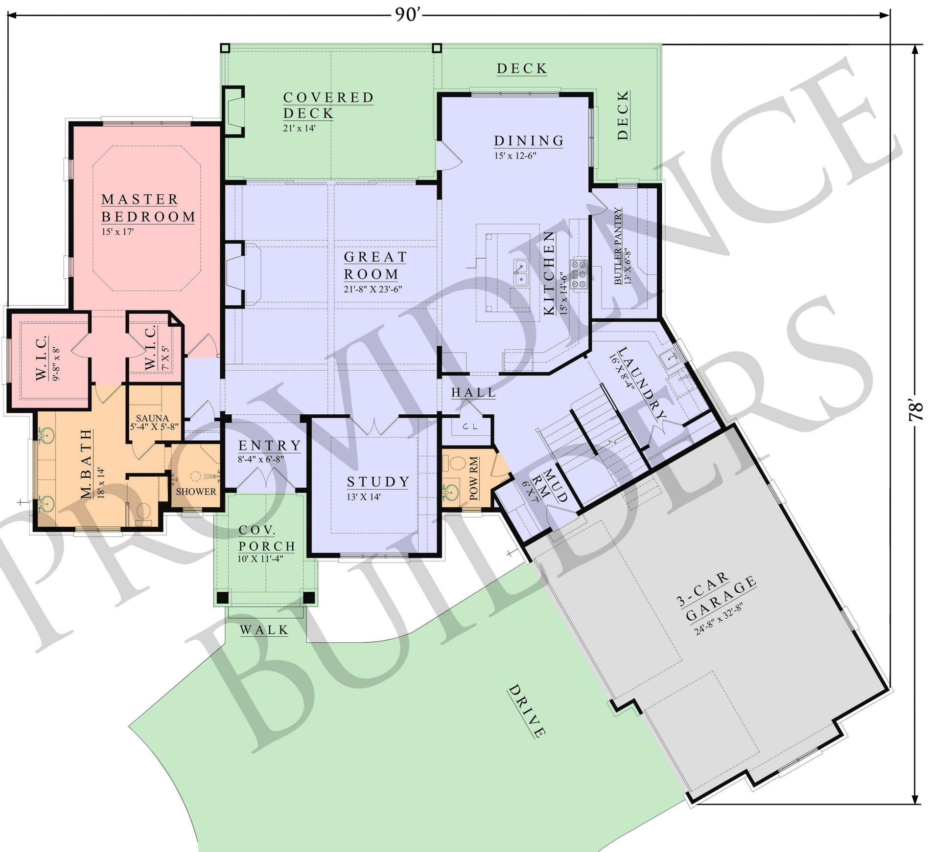
MAIN FLOOR PLAN 2504 SQ. FT.
